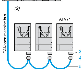
Example of CANopen diagram with SUB-D connector
