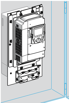
ATV71HU75N4 flush-mounted
