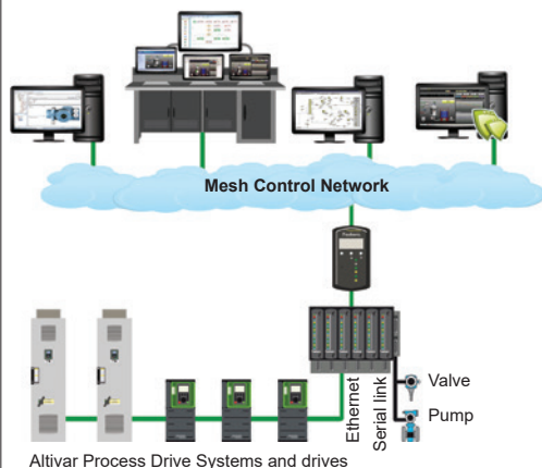
Altivar Process in EcoStruxure Foxboro DCS architecture
