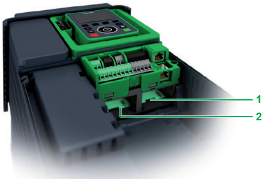
Altivar Process drives slots for additional I/O modules
